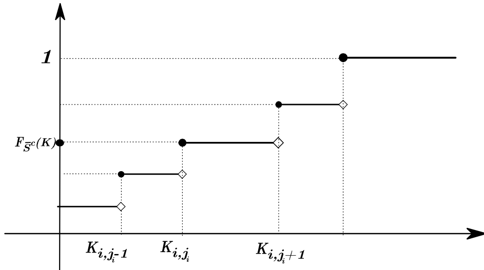
Figure 6: The cdf \overline{F}_{X_i}(x) in case i \in \overline{N}_K .
