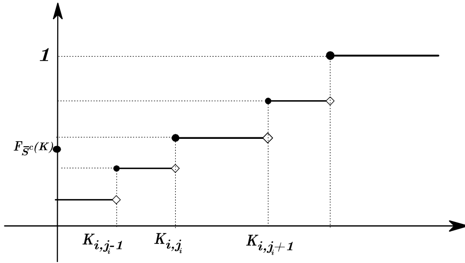
Figure 5: The cdf \overline{F}_{X_i}(x) in case i \in N_K .
